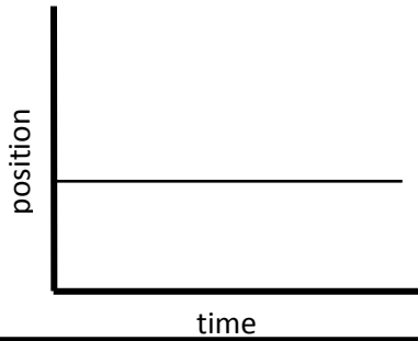
Position-Time Graph 5
