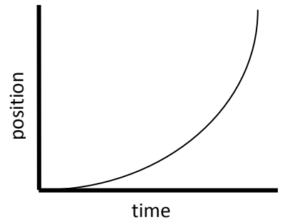
Position-Time Graph 9
