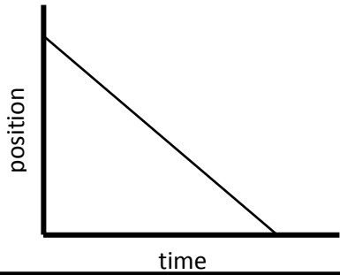
Position-Time Graph 4
