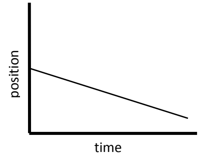
Position-Time Graph 3
