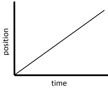
Position-Time Graph 2
