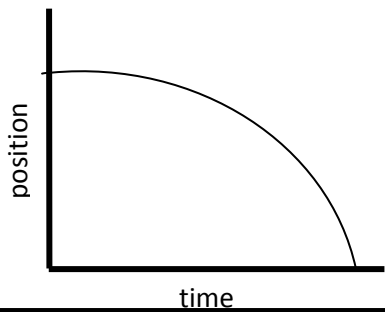
Position-Time Graph 7
