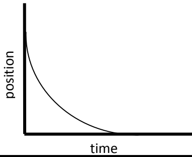
Position-Time Graph 8
