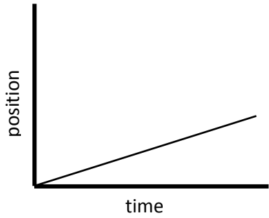
Position-Time Graph 1
